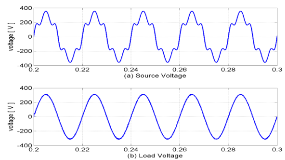
Fig 13 Series compensation for Grid voltage contains harmonics
