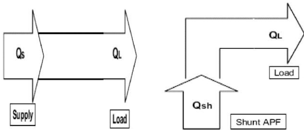
Fig 4 Reactive Power Flow No UPQC (b) Shunt APF ON
