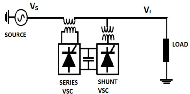
Fig.1. Block diagram of UPQC
