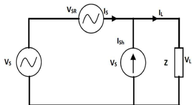
Fig.2 Equivalent circuit for UPQC
