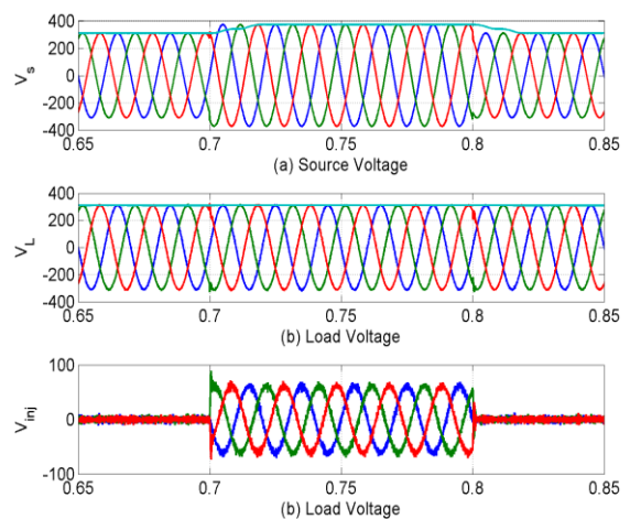
Fig 14 Mitigation of Swell in Load Voltage
