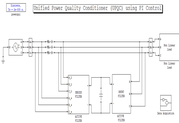
Fig10. MATLAB model of UPQC using PI Control
