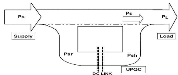
Fig.7 Active Power Flow during Normal working condition
