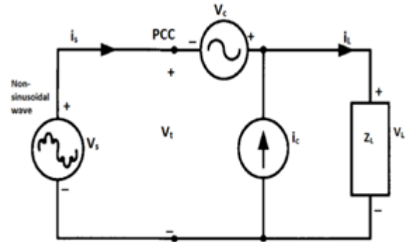
Fig 3 Left shunt UPQC compensation configuration
