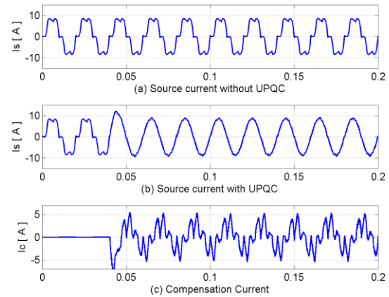
Fig 12 Shunt compensation of UPQC
