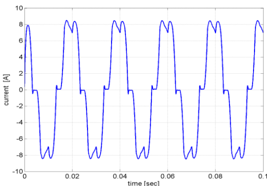
Fig 11 Source current when the compensator is not connected
