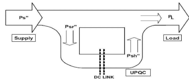
Fig. 6 Active power flow during voltage swells condition
