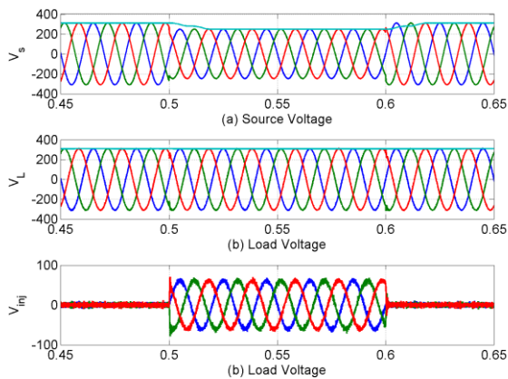
Fig 15. Mitigation of Sag in Load Voltage
