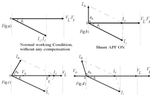
Fig 8 (a) – (d): Phasor Representation of all possible conditions
