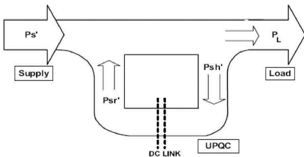
Figure 5 Active power flow during voltage sag condition
