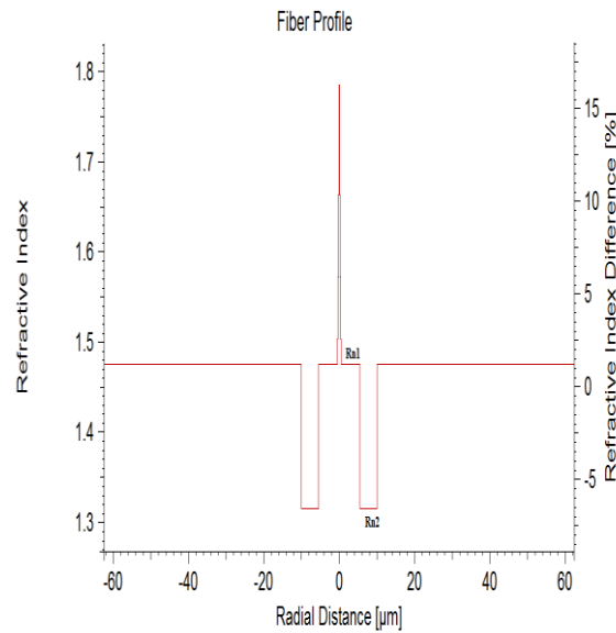
Figure (2).Exponential index profile of DCF
