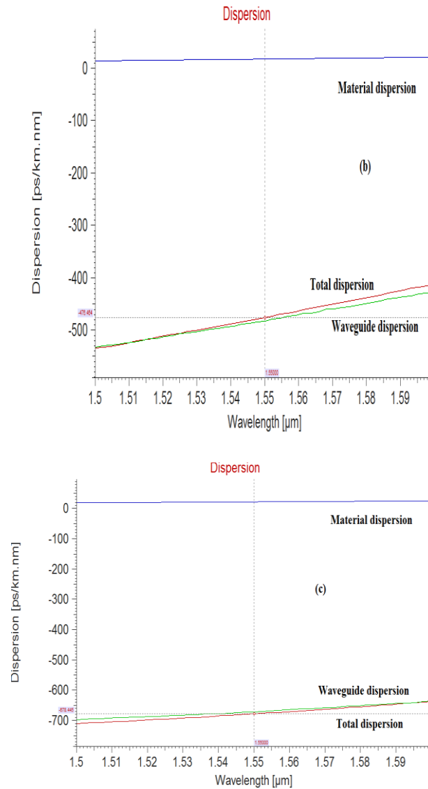
Figure (4).Dispersion of the designed DCFs (a)gaussian double index (b)exponential index (c) parabolic double index.
