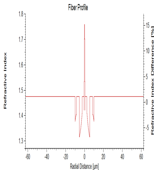
Figure (3). Parabolic double index profile of DCF
