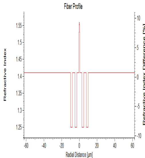
Figure (1). Gaussian double ring index profile of DCF
