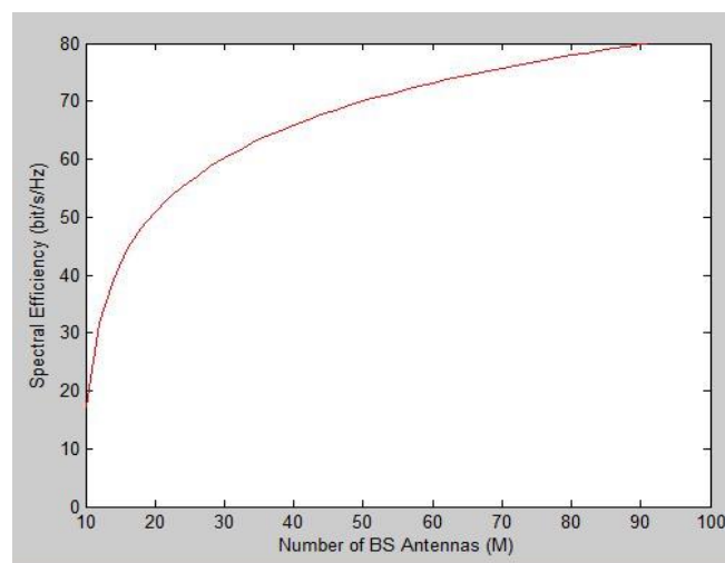
Fig. 5: Downlink Simulation with ZF Precoding
