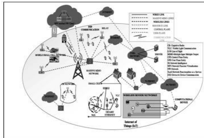
Fig. 1: General 5G cellular network architecture [5]
