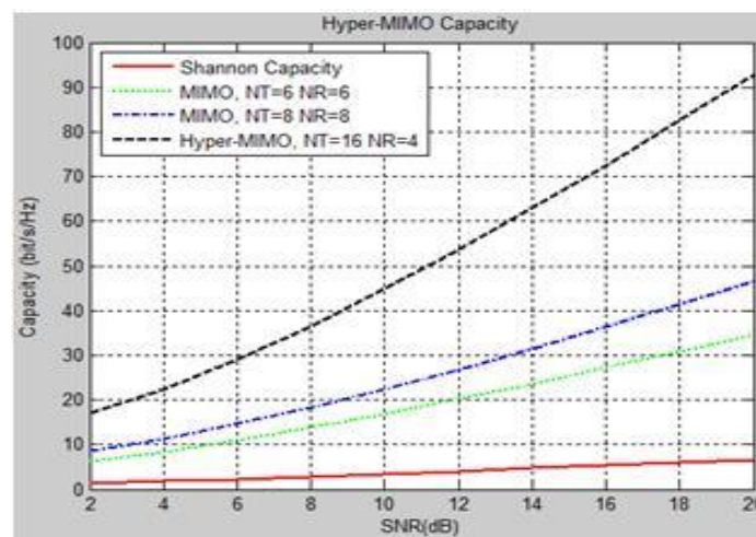
Fig. 3: Potential of Hyper-MIMO systems
