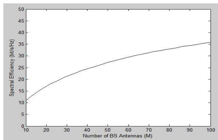
Fig. 4: Downlink Simulation with MR Precoding
